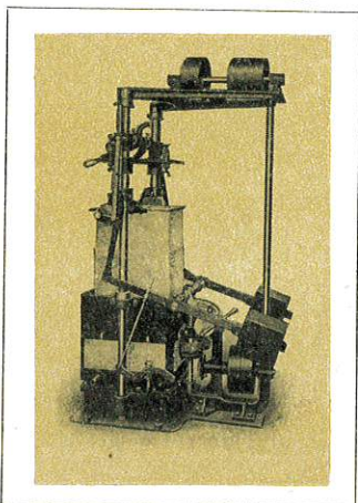
THE EICK BOTTLE WASHING & RINSING MACHINE
